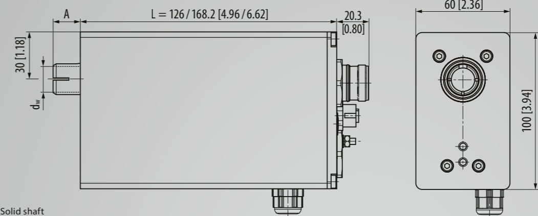
Solid shaft
