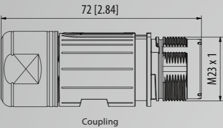
Connector type 23
