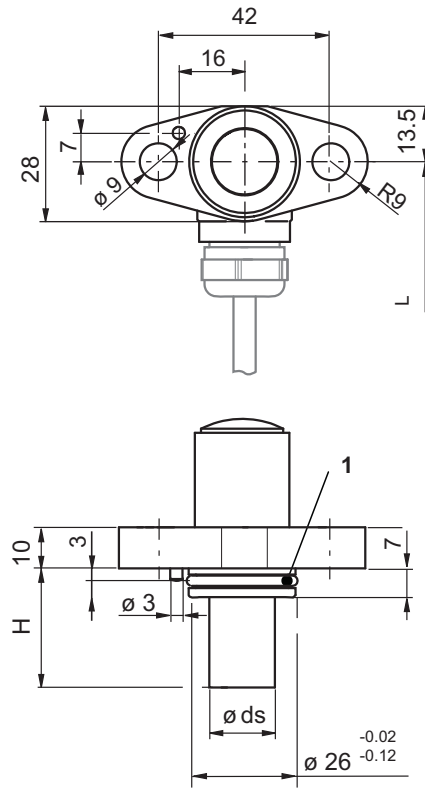
2471.....G..... Cable outlet side
