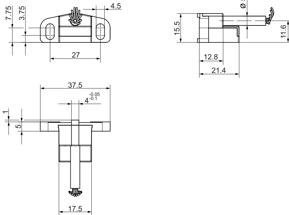
Dimensional drawing GEL 2444 with cable outlet MiniCODER (G) — axial
