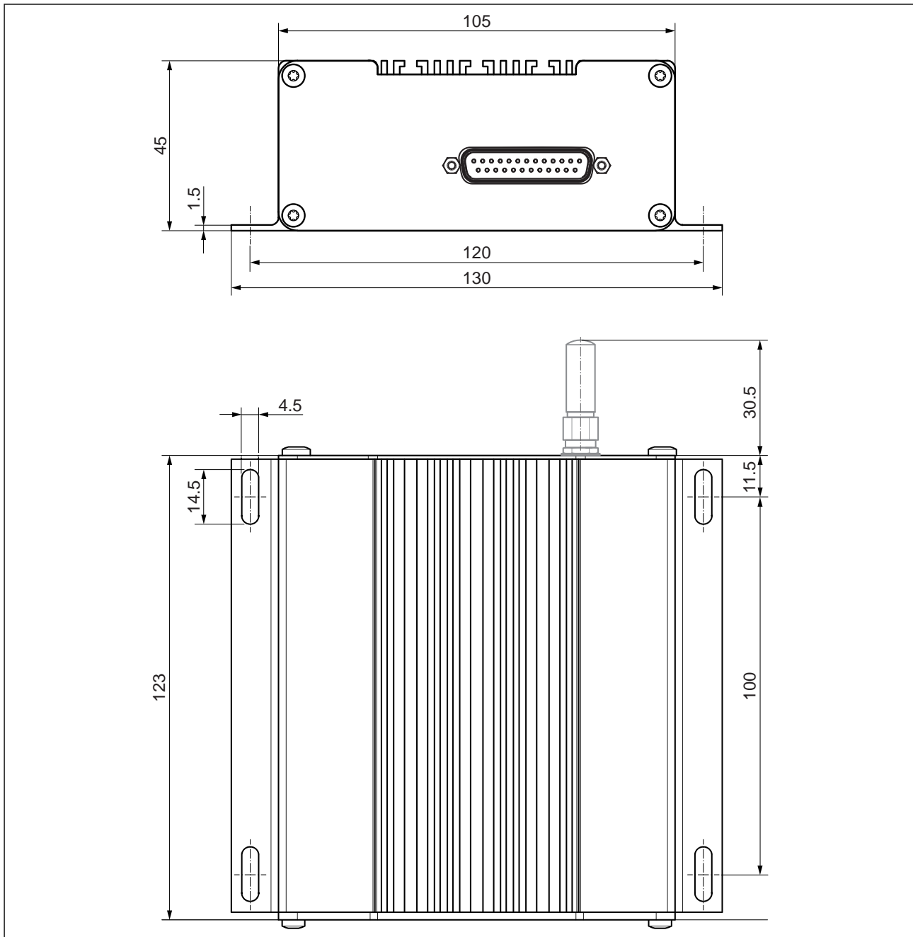
GEL 211CSR4E2D / GEL 211CSR4W2D (with WLAN antenna)
