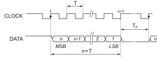
Principle of serial data transmission [RS 422 / RS 485 standard]
